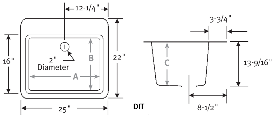
DIT 25" W x 22" D (635 mm x 559 mm) A 21-1/2", B 16", C 13-9/16" Capacity: 17-1/2 gallons
